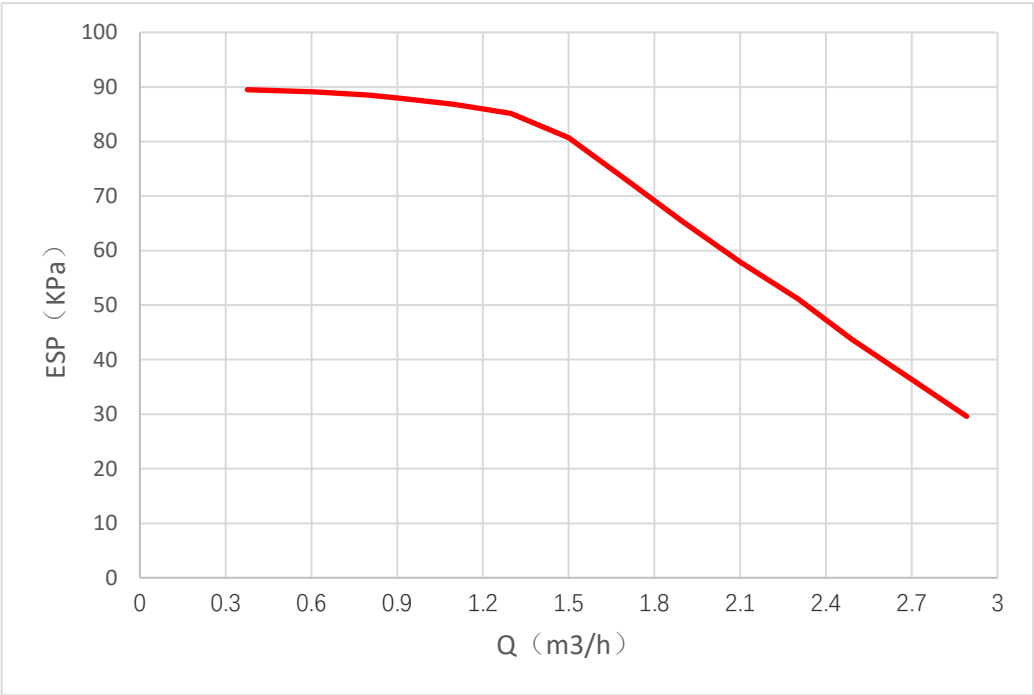
6kW hydronic performance 1
